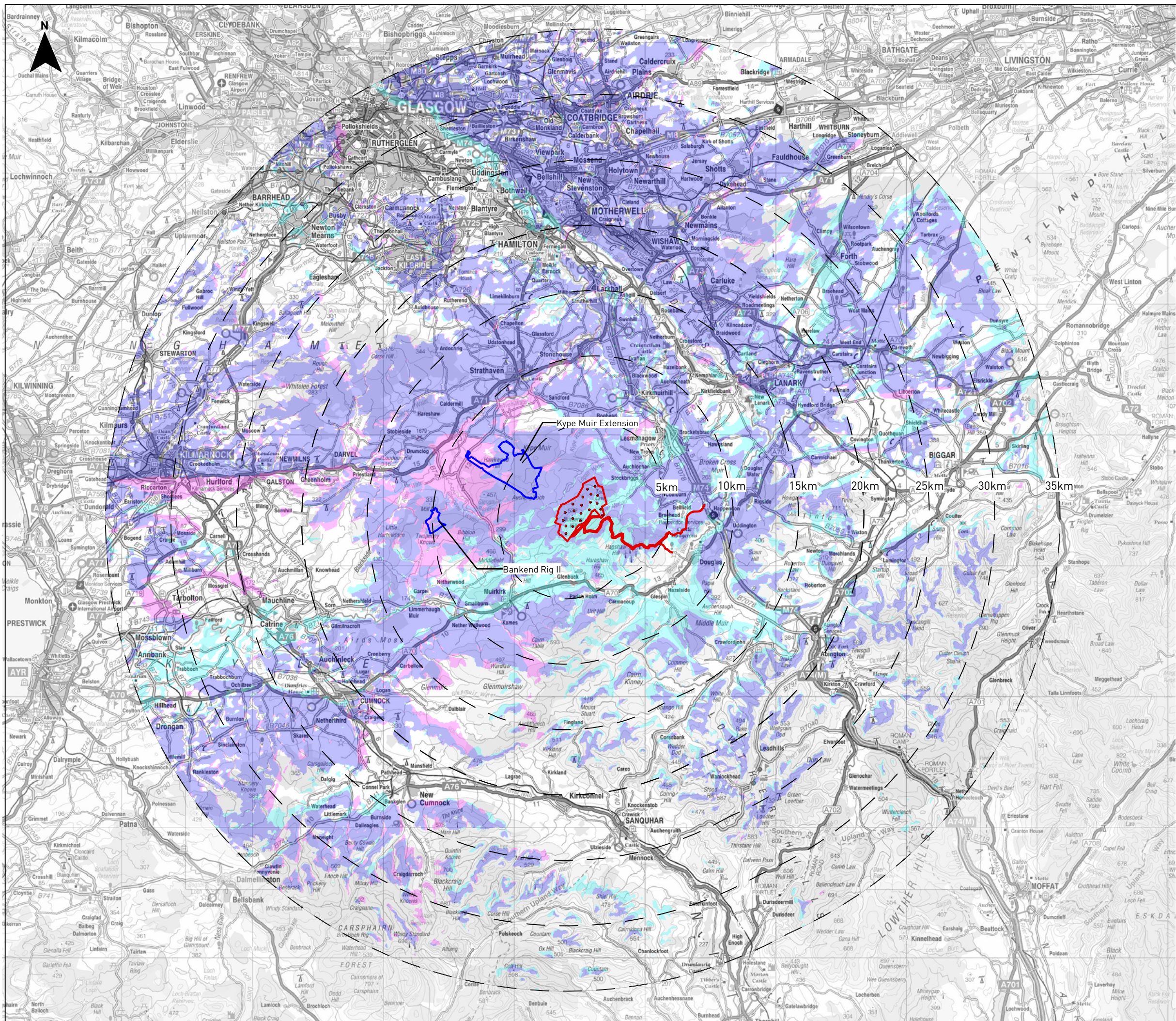
Cumberhead West Wind Farm Environmental Impact Assessment Report Figure 6.33 - Cumulative ZTV with Kype Muir Extension and Bankend Rig II
